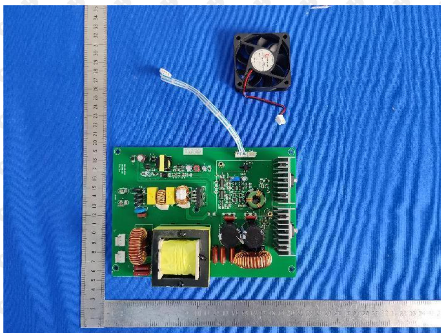
Photo 14: PCB view
