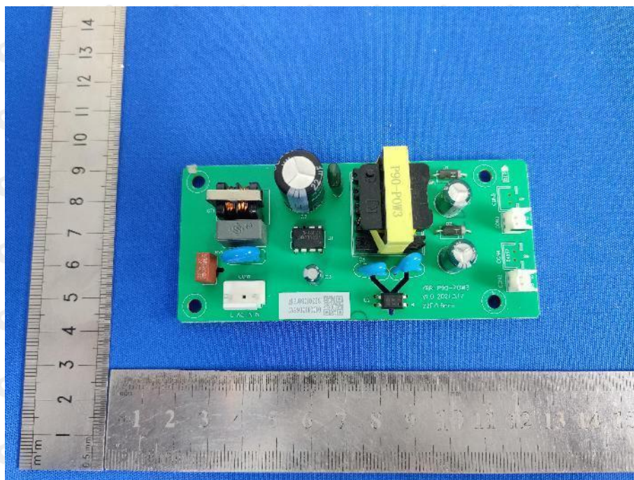
Photo 11: PCB view
