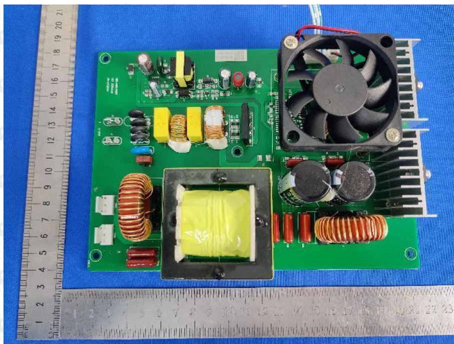
Photo 13: PCB view
