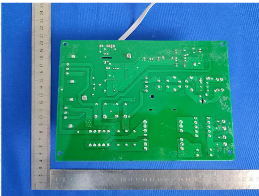
Photo 15: PCB view
